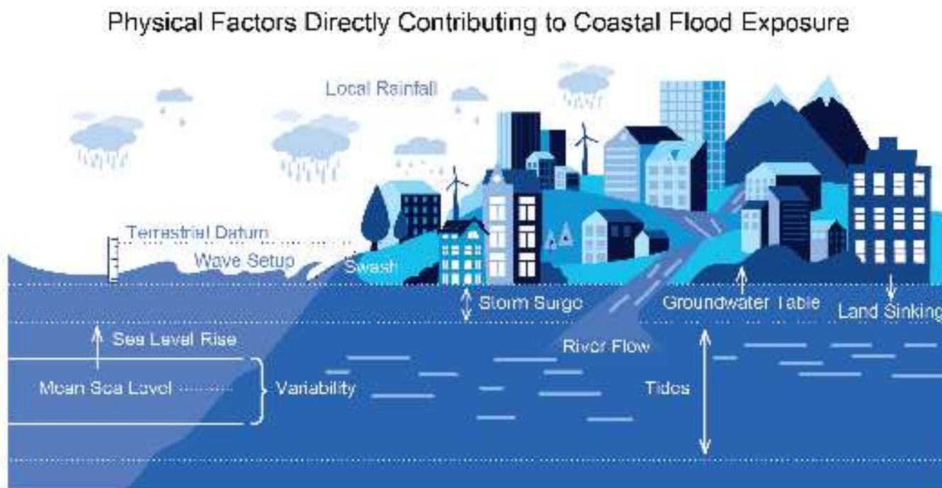
Figure 1.1: Schematic (not to scale) showing physical factors affecting coastal flood exposure. Due to the clear and strong relative sea level rise signal (i.e., combination of sea level rise and sinking lands), the probability of flooding and impacts are increasing along most U.S. coastlines.
